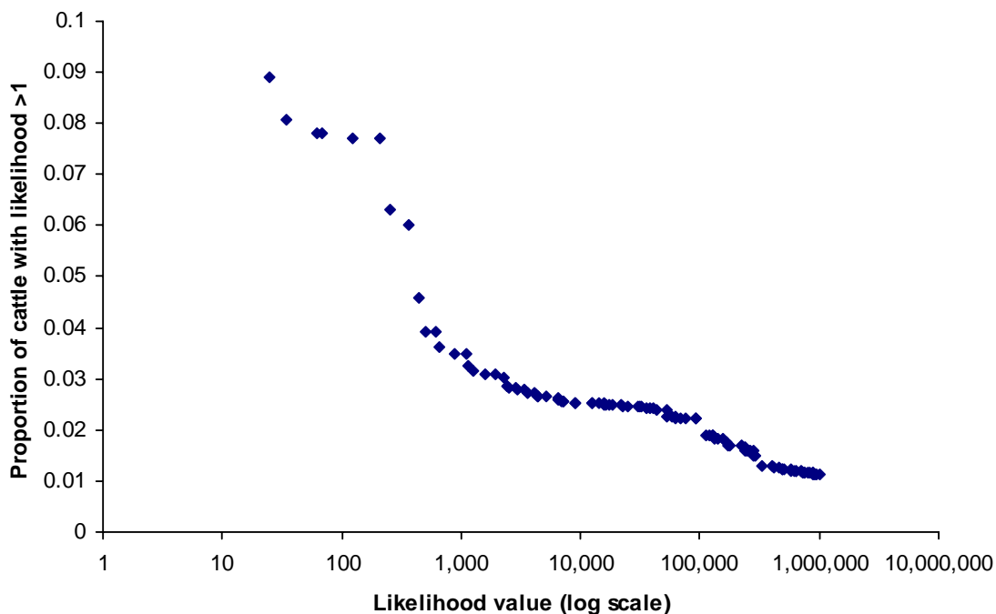
Figure 4. Plot of likelihood ratio values for cattle in the U.S. enhanced BSE surveillance database with estimated likelihood ratios greater than one.
