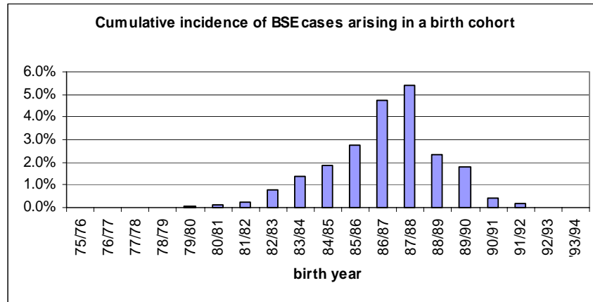
Figure 1. The cumulative lifetime incidence of BSE cases arising in a birth cohort in the U.K. (Schreuder et al. 1997). The immediate decrease in BSE cases is shown in birth cohorts born after the 1988 feed ban.
