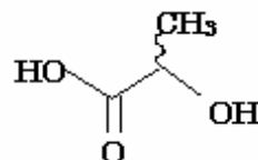
Lactic acid
