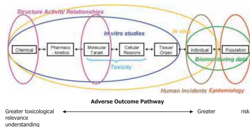
Figure C.1: Source to Outcome Pathway: Chemical effects across levels of biological organisation (adapted from NRC, 2007)
