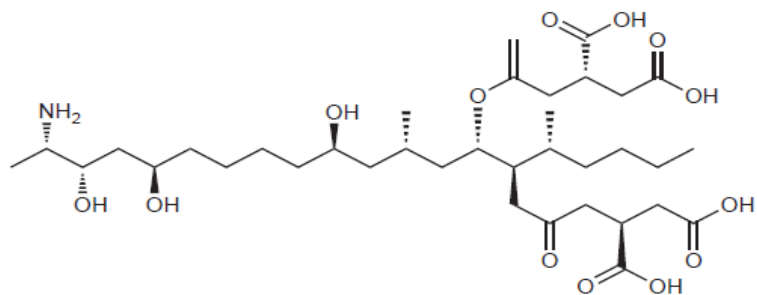
Fumonisin B 1
