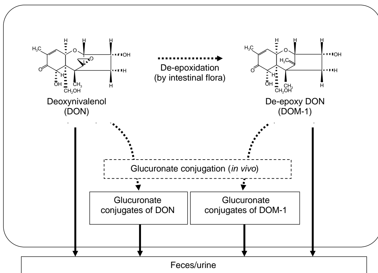
Fig. 2 Summary of major conversion and metabolic pathways of deoxynivalenol (DON)
